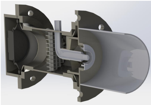
Fig. 1. Tangential combustor.
